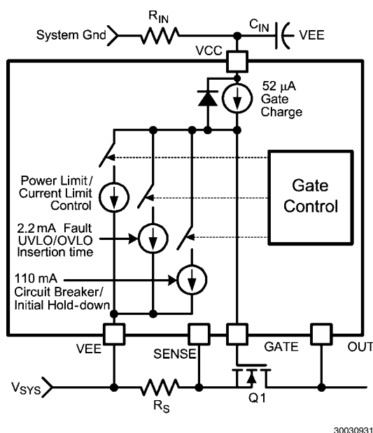
FIGURE 4. Gate Control
